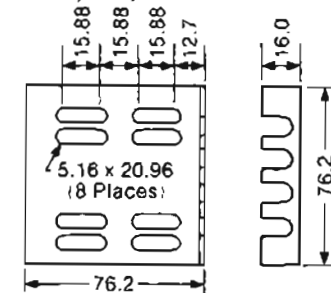
Non-HP Rack Heavy Duty Slide Bracket Kit
