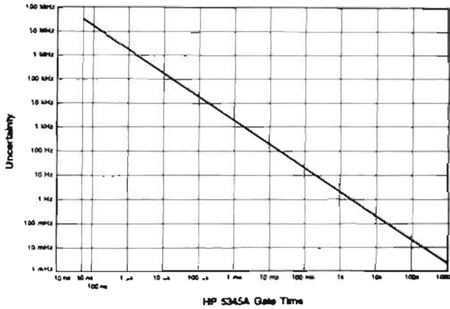
Graph 1. Uncertainty (2 x LSD) due to selected 5345A gate time.
