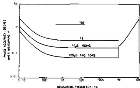
FIGURE 6: PHASE ACCURACY WHEN MEASURING L
